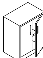
LOW SWING DOOR W=600,750,900,1050,1200 D=400,450,500,550,600 H=750,800,900
