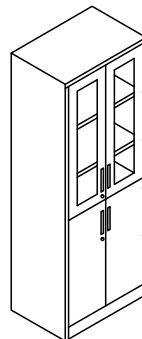
HIGH SWING DOOR WITH GLASS & WOODEN SHUTTERS W=600,750,900 D=400,450,500,550,600 H=1650,1800,2100
