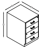
FREE STANDING PEDESTAL (4D) W=400,450 D=450,500,550,600 H=700,725,750
