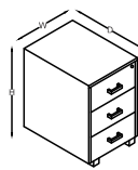
MOBILE PEDESTAL (3D) W=400,450 D=450,500,550 H=600
