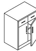
SIDE CABINET W=600,750,900 D=400,450 H=750,900
