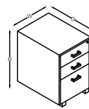
MOBILE PEDESTAL (2D1F) W=400,450 D=450,500,550 H=600,700
