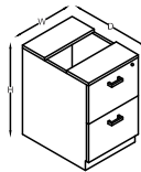
FIXED PEDESTAL (2F) W=400,450 D=450,500,550,600 H=725
