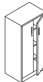
MEDIUM SWING DOOR (2S) W=600,750,900 D=400,450,500,550,600 H=1175,1200,1350,1500
