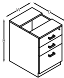
FIXED PEDESTAL (2D1F) W=400,450 D=450,500,550,600 H=725
