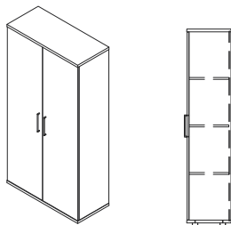
N30FST900180- 900 X 400 X 1800
