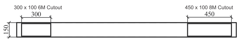
Switch Mounting Provision On Raceway For Workstation
