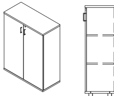
N30MST900120- 900 X 400 X 1200
