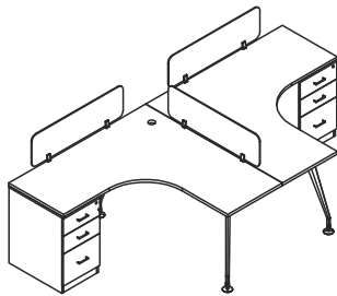
N30WSLS1S900120- 900 X 1200 X 1050 N30WSLS1S105120-1050 X 1200 X1050 N30WSLS1S120120-1200 X 1200 X 1050
